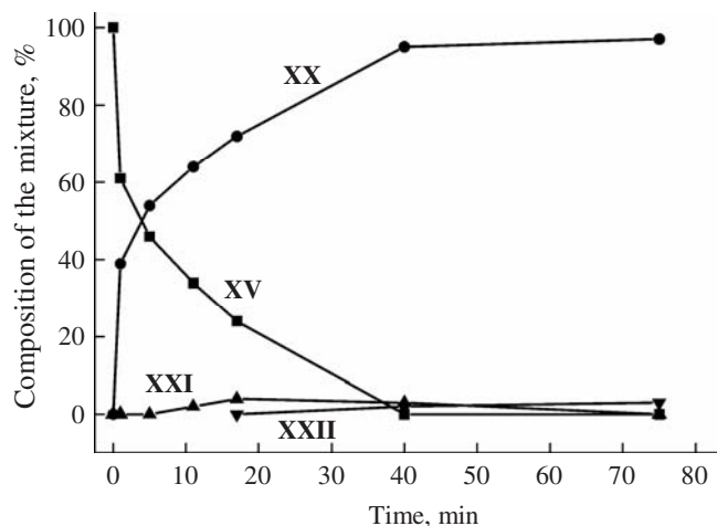
Kinetics plots for the reduction of dimethyl 2-methylidenbutanedioate ( XV ) with NaH 2 B(OPr- i ) 2 in the presence of complex VI (DMF-toluene, 17:3).
